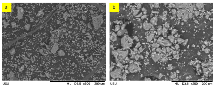
Figure 1. The morphology of (a) the volcanic ash of Mout Sinabung and (b) the extracted SiO 2
