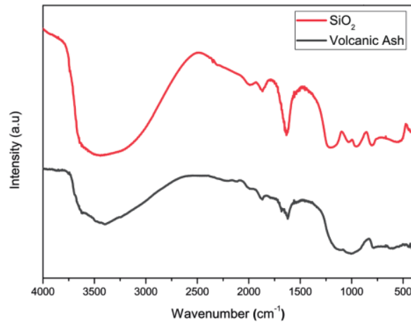
Figure 3. FTIR spectra of volcanic ash and SiO 2
