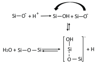
Figure 5. The reaction mechanism of SiO 2 formation
