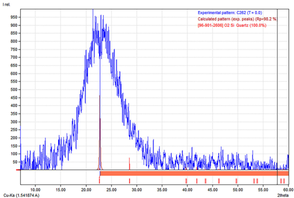
Figure 7. Diffractogram of the extracted \text{SiO}_2 from volcanic ash processed using the Match2 software
