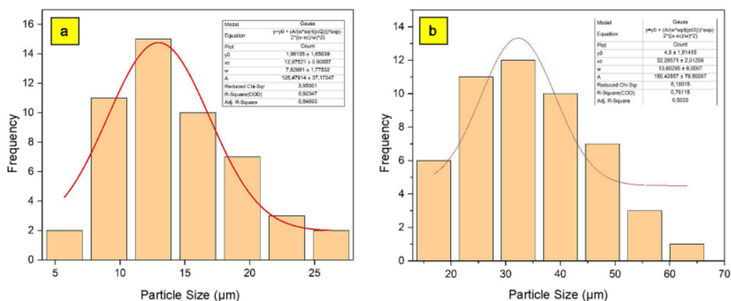
Figure 2. Particle size distribution of (a) volcanic ash sample from Mount Sinabung and (b) the extracted SiO 2
