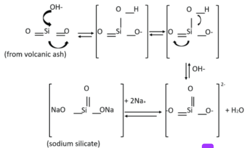
Figure 4. The reaction mechanism in the formation of sodium silicate (Na 2 SiO 3 )
