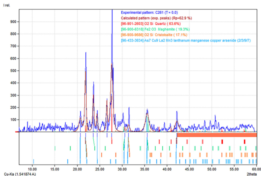
Figure 6. Diffractogram of volcanic ash processed using the Match2 software
