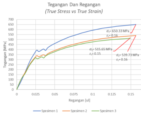
Gambar 7. Grafik True Stress – True Strain
